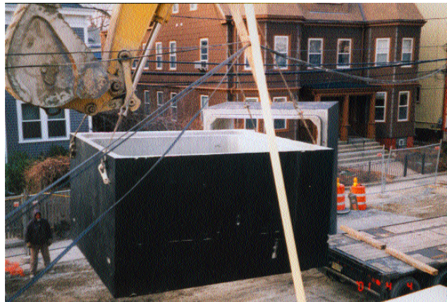
ABOVE - April 2001 One section of the concrete tank now installed below Wendell. This one, 15' high, is one of ten that make up a typical 150' tank. Tanks are now also below Holden/Scott and Museum Streets.
